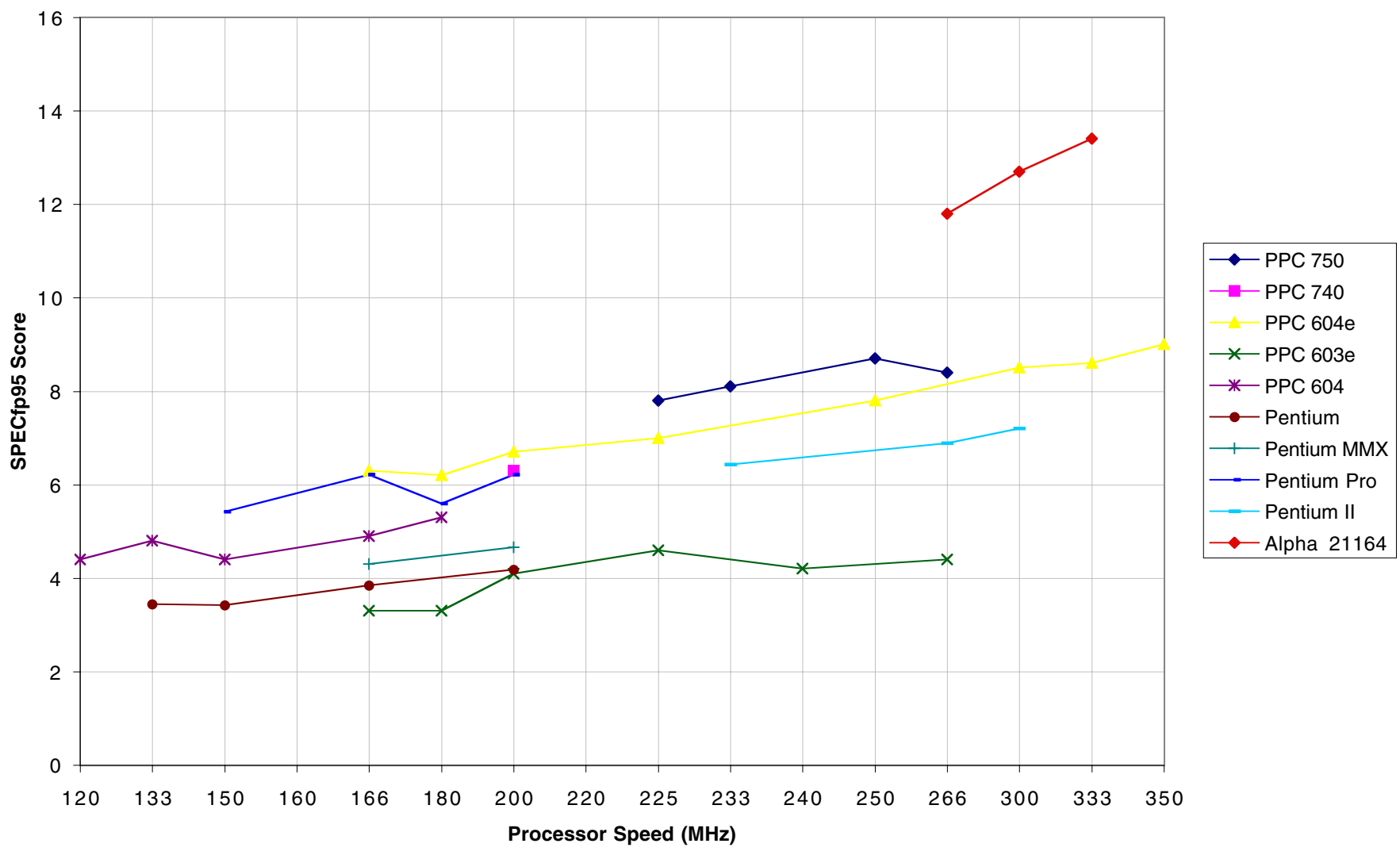
SPECfp95 comparison
