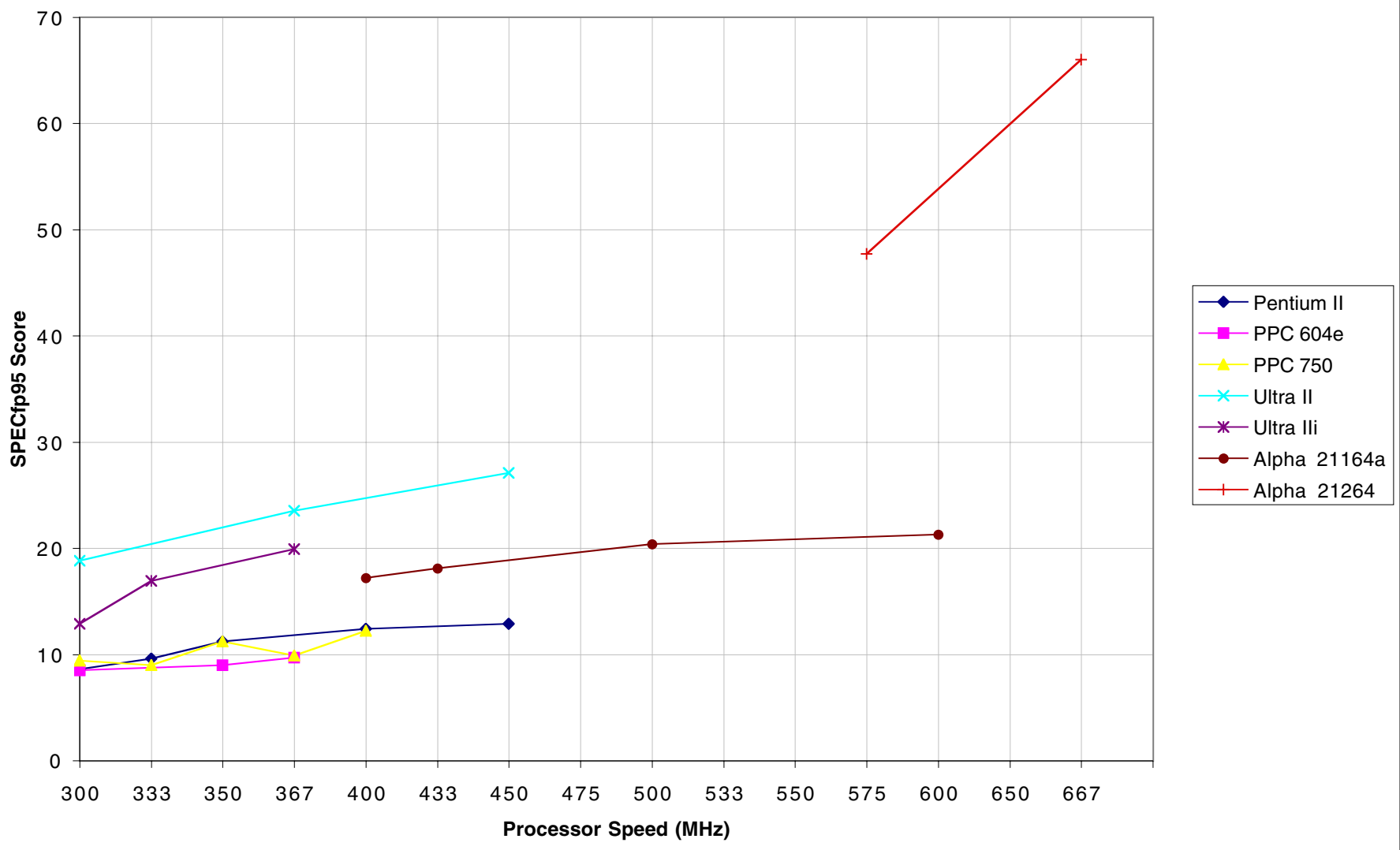
SPECfp95 comparison
